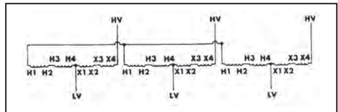
Buck-Boost Wiring Diagram 8
